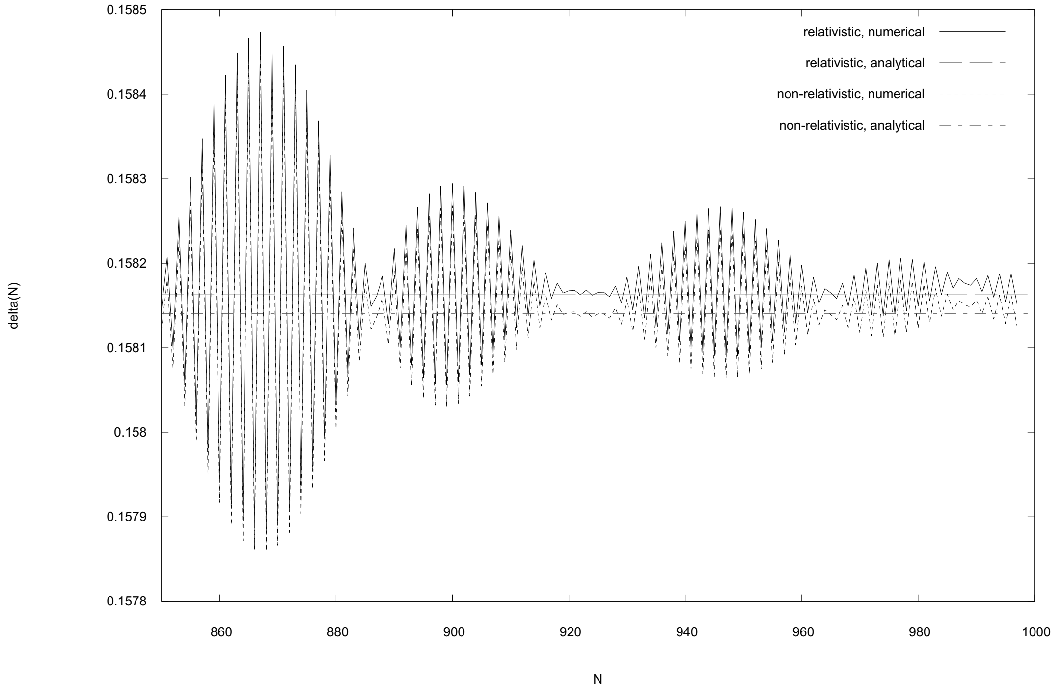
Comparison of relativistic and non-relativistic results, square-well, gaussian basis
